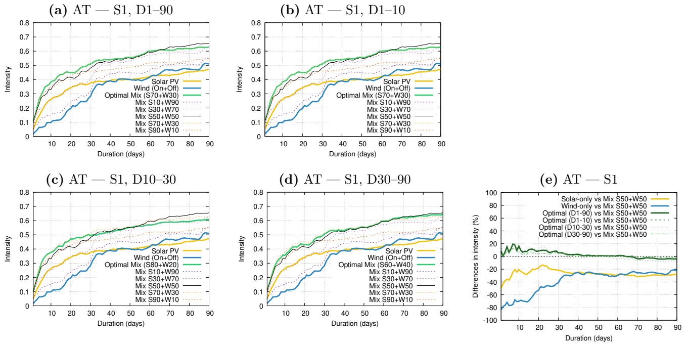
Figure 1. Panels (a–d): Intensity–Duration (ID) curves for renewable energy drought events of severity rank 1 ( S=1 ) in Austria (AT). Solar-only (yellow), wind-only (blue), and mixed capacity factor (CF) combinations are shown, with the optimal mix in green and the 50–50 mix in black (other combinations are displayed by dashed lines). Each panel shows the optima for different duration ranges: (a) D1–90, (b) D1–10, (c) D10–30 and (d) D30–90. Panel (e) displays the corresponding relative differences in drought intensity (%) between different renewable deployment configurations and the reference 50–50 solar–wind mix. Yellow and blue curves show differences between the solar-only and wind-only cases, respectively, and the 50–50 mix. Green curves show differences between the optimal mixes obtained for the four different optimized duration intervals (D1–90, D1–10, D10–30, and D30–90) and the 50–50 mix. Positive values indicate cases in which the 50–50 mix yields higher drought intensity (performs worse) than the corresponding reference configuration, while negative values indicate the opposite.
