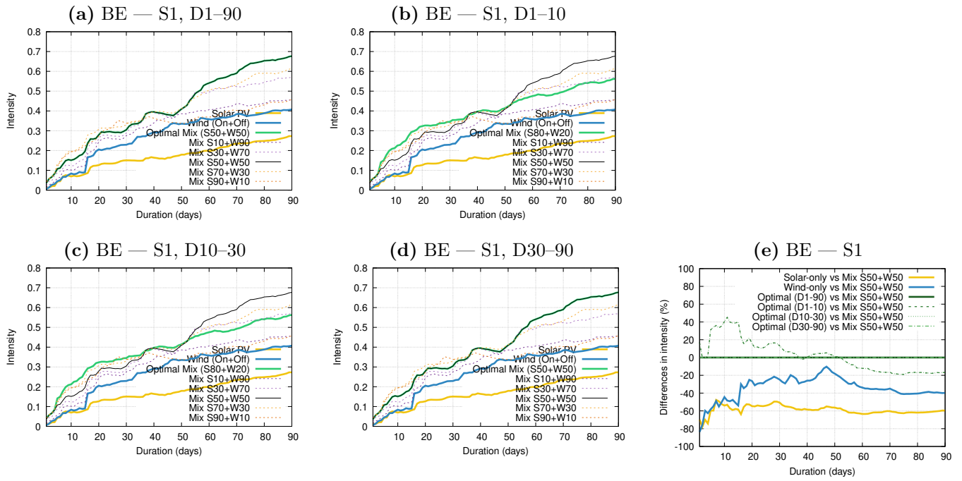
Figure 1. Panels (a–d): Intensity–Duration (ID) curves for renewable energy drought events of severity rank 1 ( S=1 ) in Belgium (BE). Solar-only (yellow), wind-only (blue), and mixed capacity factor (CF) combinations are shown, with the optimal mix in green and the 50–50 mix in black (other combinations are displayed by dashed lines). Each panel shows the optima for different duration ranges: (a) D1–90, (b) D1–10, (c) D10–30 and (d) D30–90. Panel (e) displays the corresponding relative differences in drought intensity (%) between different renewable deployment configurations and the reference 50–50 solar–wind mix. Yellow and blue curves show differences between the solar-only and wind-only cases, respectively, and the 50–50 mix. Green curves show differences between the optimal mixes obtained for the four different optimized duration intervals (D1–90, D1–10, D10–30, and D30–90) and the 50–50 mix. Positive values indicate cases in which the 50–50 mix yields higher drought intensity (performs worse) than the corresponding reference configuration, while negative values indicate the opposite.
