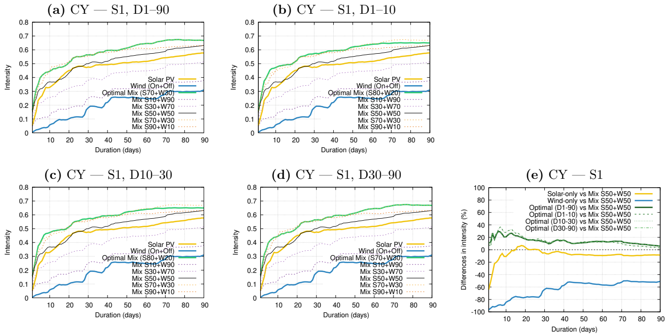
Figure 1. Panels (a–d): Intensity–Duration (ID) curves for renewable energy drought events of severity rank 1 ( S=1 ) in Cyprus (CY). Solar-only (yellow), wind-only (blue), and mixed capacity factor (CF) combinations are shown, with the optimal mix in green and the 50–50 mix in black (other combinations are displayed by dashed lines). Each panel shows the optima for different duration ranges: (a) D1–90, (b) D1–10, (c) D10–30 and (d) D30–90. Panel (e) displays the corresponding relative differences in drought intensity (%) between different renewable deployment configurations and the reference 50–50 solar–wind mix. Yellow and blue curves show differences between the solar-only and wind-only cases, respectively, and the 50–50 mix. Green curves show differences between the optimal mixes obtained for the four different optimized duration intervals (D1–90, D1–10, D10–30, and D30–90) and the 50–50 mix. Positive values indicate cases in which the 50–50 mix yields higher drought intensity (performs worse) than the corresponding reference configuration, while negative values indicate the opposite.
