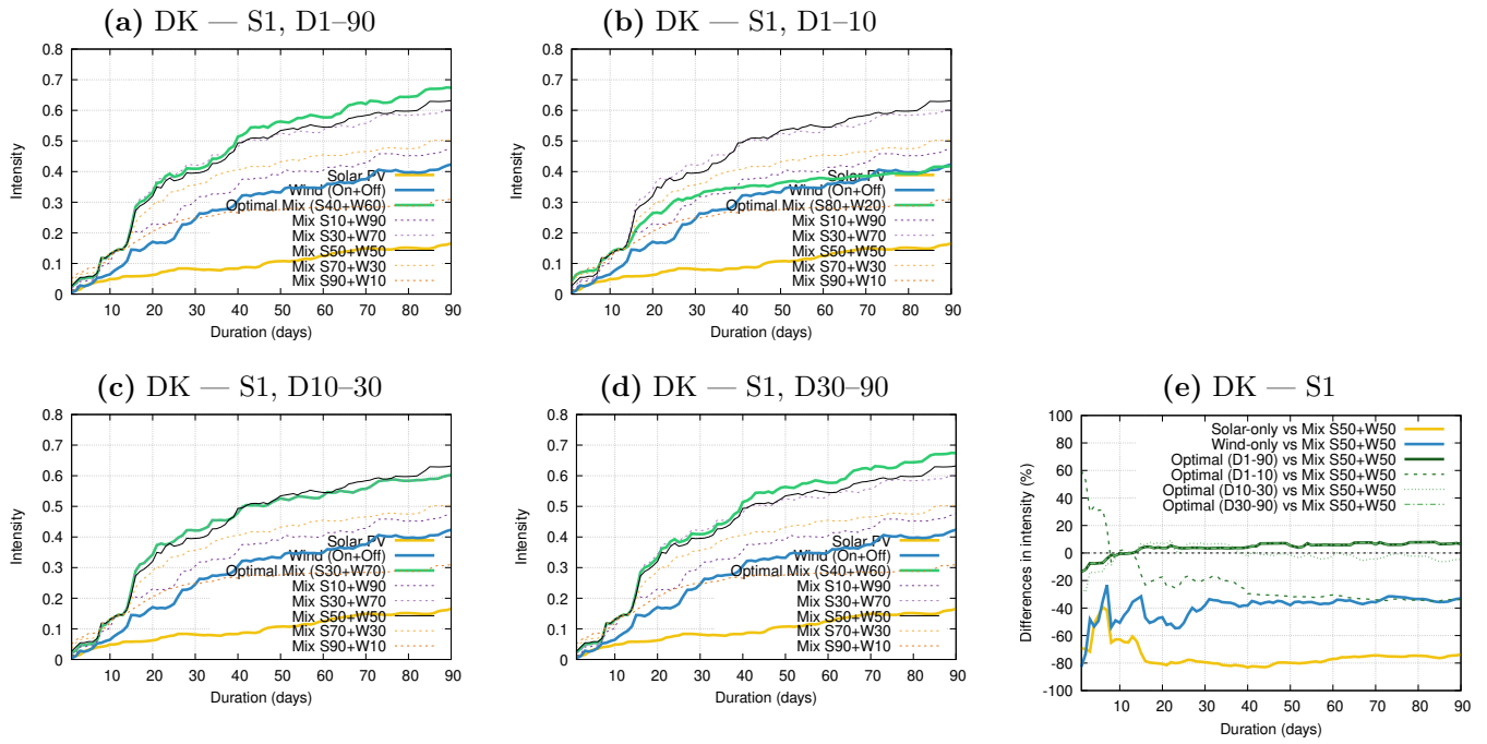
Figure 1. Panels (a–d): Intensity–Duration (ID) curves for renewable energy drought events of severity rank 1 ( S=1 ) in Denmark (DK). Solar-only (yellow), wind-only (blue), and mixed capacity factor (CF) combinations are shown, with the optimal mix in green and the 50–50 mix in black (other combinations are displayed by dashed lines). Each panel shows the optima for different duration ranges: (a) D1–90, (b) D1–10, (c) D10–30 and (d) D30–90. Panel (e) displays the corresponding relative differences in drought intensity (%) between different renewable deployment configurations and the reference 50–50 solar–wind mix. Yellow and blue curves show differences between the solar-only and wind-only cases, respectively, and the 50–50 mix. Green curves show differences between the optimal mixes obtained for the four different optimized duration intervals (D1–90, D1–10, D10–30, and D30–90) and the 50–50 mix. Positive values indicate cases in which the 50–50 mix yields higher drought intensity (performs worse) than the corresponding reference configuration, while negative values indicate the opposite.
