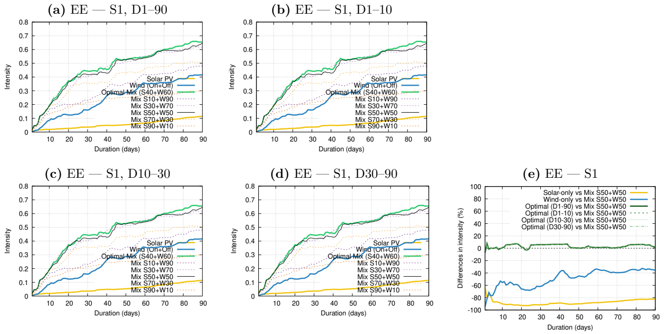
Figure 1. Panels (a–d): Intensity–Duration (ID) curves for renewable energy drought events of severity rank 1 ( S=1 ) in Estonia (EE). Solar-only (yellow), wind-only (blue), and mixed capacity factor (CF) combinations are shown, with the optimal mix in green and the 50–50 mix in black (other combinations are displayed by dashed lines). Each panel shows the optima for different duration ranges: (a) D1–90, (b) D1–10, (c) D10–30 and (d) D30–90. Panel (e) displays the corresponding relative differences in drought intensity (%) between different renewable deployment configurations and the reference 50–50 solar–wind mix. Yellow and blue curves show differences between the solar-only and wind-only cases, respectively, and the 50–50 mix. Green curves show differences between the optimal mixes obtained for the four different optimized duration intervals (D1–90, D1–10, D10–30, and D30–90) and the 50–50 mix. Positive values indicate cases in which the 50–50 mix yields higher drought intensity (performs worse) than the corresponding reference configuration, while negative values indicate the opposite.
