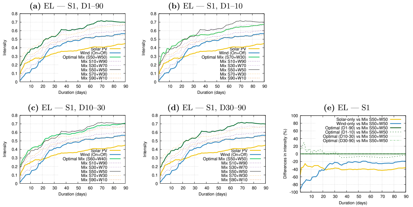
Figure 1. Panels (a–d): Intensity–Duration (ID) curves for renewable energy drought events of severity rank 1 ( S=1 ) in Greece (EL). Solar-only (yellow), wind-only (blue), and mixed capacity factor (CF) combinations are shown, with the optimal mix in green and the 50–50 mix in black (other combinations are displayed by dashed lines). Each panel shows the optima for different duration ranges: (a) D1–90, (b) D1–10, (c) D10–30 and (d) D30–90. Panel (e) displays the corresponding relative differences in drought intensity (%) between different renewable deployment configurations and the reference 50–50 solar–wind mix. Yellow and blue curves show differences between the solar-only and wind-only cases, respectively, and the 50–50 mix. Green curves show differences between the optimal mixes obtained for the four different optimized duration intervals (D1–90, D1–10, D10–30, and D30–90) and the 50–50 mix. Positive values indicate cases in which the 50–50 mix yields higher drought intensity (performs worse) than the corresponding reference configuration, while negative values indicate the opposite.
