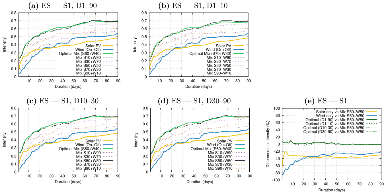
Figure 1. Panels (a–d): Intensity–Duration (ID) curves for renewable energy drought events of severity rank 1 ( S=1 ) in Spain (ES). Solar-only (yellow), wind-only (blue), and mixed capacity factor (CF) combinations are shown, with the optimal mix in green and the 50–50 mix in black (other combinations are displayed by dashed lines). Each panel shows the optima for different duration ranges: (a) D1–90, (b) D1–10, (c) D10–30 and (d) D30–90. Panel (e) displays the corresponding relative differences in drought intensity (%) between different renewable deployment configurations and the reference 50–50 solar–wind mix. Yellow and blue curves show differences between the solar-only and wind-only cases, respectively, and the 50–50 mix. Green curves show differences between the optimal mixes obtained for the four different optimized duration intervals (D1–90, D1–10, D10–30, and D30–90) and the 50–50 mix. Positive values indicate cases in which the 50–50 mix yields higher drought intensity (performs worse) than the corresponding reference configuration, while negative values indicate the opposite.
