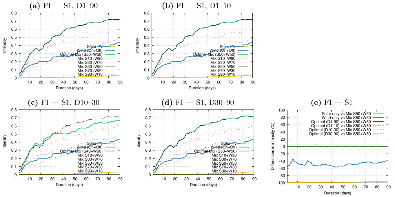
Figure 1. Panels (a–d): Intensity–Duration (ID) curves for renewable energy drought events of severity rank 1 ( S=1 ) in Finland (FI). Solar-only (yellow), wind-only (blue), and mixed capacity factor (CF) combinations are shown, with the optimal mix in green and the 50–50 mix in black (other combinations are displayed by dashed lines). Each panel shows the optima for different duration ranges: (a) D1–90, (b) D1–10, (c) D10–30 and (d) D30–90. Panel (e) displays the corresponding relative differences in drought intensity (%) between different renewable deployment configurations and the reference 50–50 solar–wind mix. Yellow and blue curves show differences between the solar-only and wind-only cases, respectively, and the 50–50 mix. Green curves show differences between the optimal mixes obtained for the four different optimized duration intervals (D1–90, D1–10, D10–30, and D30–90) and the 50–50 mix. Positive values indicate cases in which the 50–50 mix yields higher drought intensity (performs worse) than the corresponding reference configuration, while negative values indicate the opposite.
