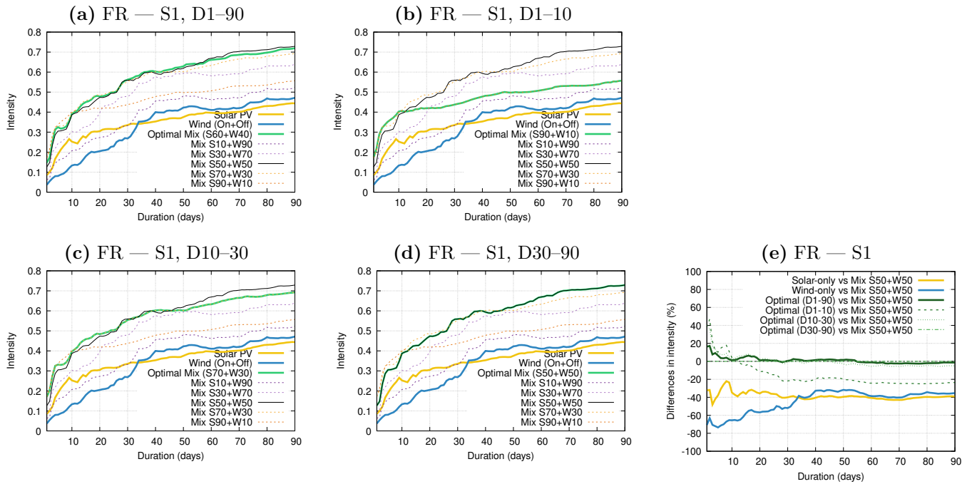
Figure 1. Panels (a–d): Intensity–Duration (ID) curves for renewable energy drought events of severity rank 1 ( S=1 ) in France (FR). Solar-only (yellow), wind-only (blue), and mixed capacity factor (CF) combinations are shown, with the optimal mix in green and the 50–50 mix in black (other combinations are displayed by dashed lines). Each panel shows the optima for different duration ranges: (a) D1–90, (b) D1–10, (c) D10–30 and (d) D30–90. Panel (e) displays the corresponding relative differences in drought intensity (%) between different renewable deployment configurations and the reference 50–50 solar–wind mix. Yellow and blue curves show differences between the solar-only and wind-only cases, respectively, and the 50–50 mix. Green curves show differences between the optimal mixes obtained for the four different optimized duration intervals (D1–90, D1–10, D10–30, and D30–90) and the 50–50 mix. Positive values indicate cases in which the 50–50 mix yields higher drought intensity (performs worse) than the corresponding reference configuration, while negative values indicate the opposite.
