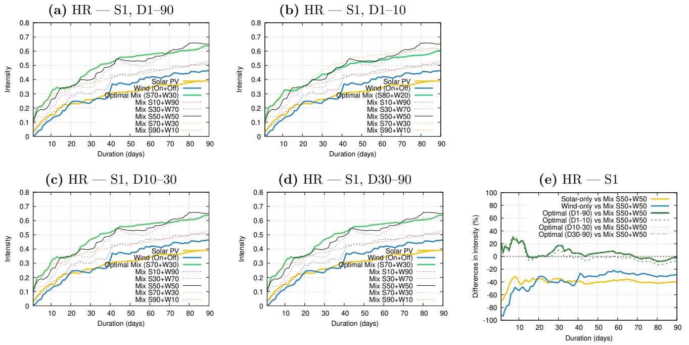
Figure 1. Panels (a–d): Intensity–Duration (ID) curves for renewable energy drought events of severity rank 1 ( S=1 ) in Croatia (HR). Solar-only (yellow), wind-only (blue), and mixed capacity factor (CF) combinations are shown, with the optimal mix in green and the 50–50 mix in black (other combinations are displayed by dashed lines). Each panel shows the optima for different duration ranges: (a) D1–90, (b) D1–10, (c) D10–30 and (d) D30–90. Panel (e) displays the corresponding relative differences in drought intensity (%) between different renewable deployment configurations and the reference 50–50 solar–wind mix. Yellow and blue curves show differences between the solar-only and wind-only cases, respectively, and the 50–50 mix. Green curves show differences between the optimal mixes obtained for the four different optimized duration intervals (D1–90, D1–10, D10–30, and D30–90) and the 50–50 mix. Positive values indicate cases in which the 50–50 mix yields higher drought intensity (performs worse) than the corresponding reference configuration, while negative values indicate the opposite.
