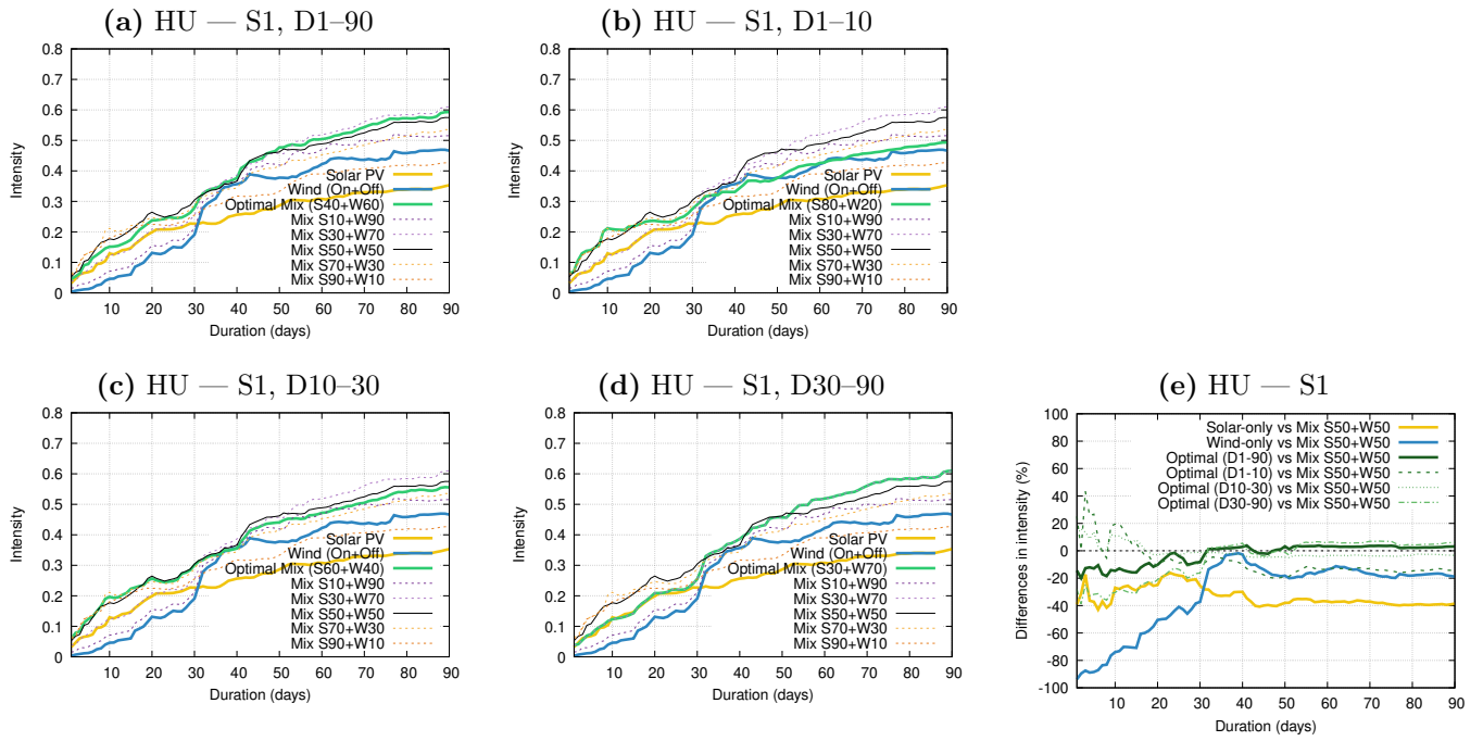
Figure 1. Panels (a–d): Intensity–Duration (ID) curves for renewable energy drought events of severity rank 1 ( S=1 ) in Hungary (HU). Solar-only (yellow), wind-only (blue), and mixed capacity factor (CF) combinations are shown, with the optimal mix in green and the 50–50 mix in black (other combinations are displayed by dashed lines). Each panel shows the optima for different duration ranges: (a) D1–90, (b) D1–10, (c) D10–30 and (d) D30–90. Panel (e) displays the corresponding relative differences in drought intensity (%) between different renewable deployment configurations and the reference 50–50 solar–wind mix. Yellow and blue curves show differences between the solar-only and wind-only cases, respectively, and the 50–50 mix. Green curves show differences between the optimal mixes obtained for the four different optimized duration intervals (D1–90, D1–10, D10–30, and D30–90) and the 50–50 mix. Positive values indicate cases in which the 50–50 mix yields higher drought intensity (performs worse) than the corresponding reference configuration, while negative values indicate the opposite.
