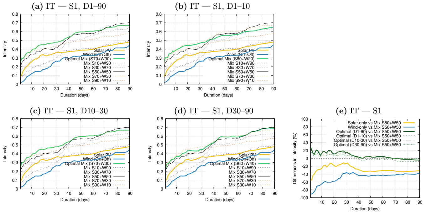
Figure 1. Panels (a–d): Intensity–Duration (ID) curves for renewable energy drought events of severity rank 1 ( S=1 ) in Italy (IT). Solar-only (yellow), wind-only (blue), and mixed capacity factor (CF) combinations are shown, with the optimal mix in green and the 50–50 mix in black (other combinations are displayed by dashed lines). Each panel shows the optima for different duration ranges: (a) D1–90, (b) D1–10, (c) D10–30 and (d) D30–90. Panel (e) displays the corresponding relative differences in drought intensity (%) between different renewable deployment configurations and the reference 50–50 solar–wind mix. Yellow and blue curves show differences between the solar-only and wind-only cases, respectively, and the 50–50 mix. Green curves show differences between the optimal mixes obtained for the four different optimized duration intervals (D1–90, D1–10, D10–30, and D30–90) and the 50–50 mix. Positive values indicate cases in which the 50–50 mix yields higher drought intensity (performs worse) than the corresponding reference configuration, while negative values indicate the opposite.
