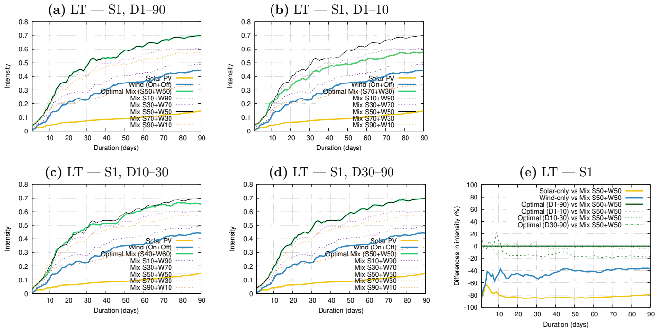
Figure 1. Panels (a–d): Intensity–Duration (ID) curves for renewable energy drought events of severity rank 1 ( S=1 ) in Lithuania (LT). Solar-only (yellow), wind-only (blue), and mixed capacity factor (CF) combinations are shown, with the optimal mix in green and the 50–50 mix in black (other combinations are displayed by dashed lines). Each panel shows the optima for different duration ranges: (a) D1–90, (b) D1–10, (c) D10–30 and (d) D30–90. Panel (e) displays the corresponding relative differences in drought intensity (%) between different renewable deployment configurations and the reference 50–50 solar–wind mix. Yellow and blue curves show differences between the solar-only and wind-only cases, respectively, and the 50–50 mix. Green curves show differences between the optimal mixes obtained for the four different optimized duration intervals (D1–90, D1–10, D10–30, and D30–90) and the 50–50 mix. Positive values indicate cases in which the 50–50 mix yields higher drought intensity (performs worse) than the corresponding reference configuration, while negative values indicate the opposite.
