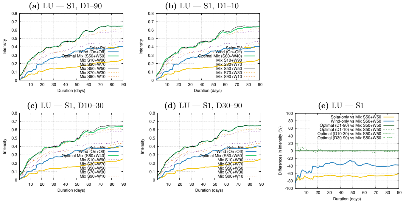
Figure 1. Panels (a–d): Intensity–Duration (ID) curves for renewable energy drought events of severity rank 1 ( S=1 ) in Luxembourg (LU). Solar-only (yellow), wind-only (blue), and mixed capacity factor (CF) combinations are shown, with the optimal mix in green and the 50–50 mix in black (other combinations are displayed by dashed lines). Each panel shows the optima for different duration ranges: (a) D1–90, (b) D1–10, (c) D10–30 and (d) D30–90. Panel (e) displays the corresponding relative differences in drought intensity (%) between different renewable deployment configurations and the reference 50–50 solar–wind mix. Yellow and blue curves show differences between the solar-only and wind-only cases, respectively, and the 50–50 mix. Green curves show differences between the optimal mixes obtained for the four different optimized duration intervals (D1–90, D1–10, D10–30, and D30–90) and the 50–50 mix. Positive values indicate cases in which the 50–50 mix yields higher drought intensity (performs worse) than the corresponding reference configuration, while negative values indicate the opposite.
