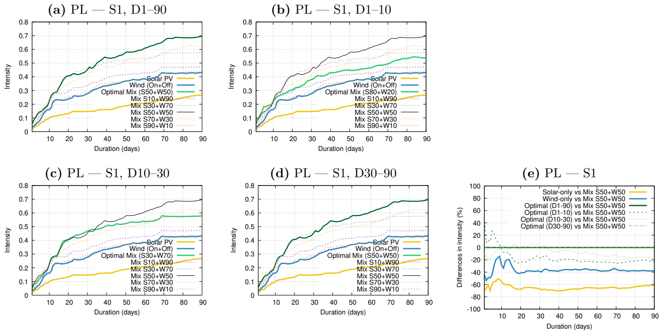
Figure 1. Panels (a–d): Intensity–Duration (ID) curves for renewable energy drought events of severity rank 1 ( S=1 ) in Poland (PL). Solar-only (yellow), wind-only (blue), and mixed capacity factor (CF) combinations are shown, with the optimal mix in green and the 50–50 mix in black (other combinations are displayed by dashed lines). Each panel shows the optima for different duration ranges: (a) D1–90, (b) D1–10, (c) D10–30 and (d) D30–90. Panel (e) displays the corresponding relative differences in drought intensity (%) between different renewable deployment configurations and the reference 50–50 solar–wind mix. Yellow and blue curves show differences between the solar-only and wind-only cases, respectively, and the 50–50 mix. Green curves show differences between the optimal mixes obtained for the four different optimized duration intervals (D1–90, D1–10, D10–30, and D30–90) and the 50–50 mix. Positive values indicate cases in which the 50–50 mix yields higher drought intensity (performs worse) than the corresponding reference configuration, while negative values indicate the opposite.
