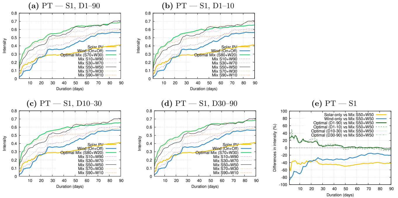
Figure 1. Panels (a–d): Intensity–Duration (ID) curves for renewable energy drought events of severity rank 1 ( S=1 ) in Portugal (PT). Solar-only (yellow), wind-only (blue), and mixed capacity factor (CF) combinations are shown, with the optimal mix in green and the 50–50 mix in black (other combinations are displayed by dashed lines). Each panel shows the optima for different duration ranges: (a) D1–90, (b) D1–10, (c) D10–30 and (d) D30–90. Panel (e) displays the corresponding relative differences in drought intensity (%) between different renewable deployment configurations and the reference 50–50 solar–wind mix. Yellow and blue curves show differences between the solar-only and wind-only cases, respectively, and the 50–50 mix. Green curves show differences between the optimal mixes obtained for the four different optimized duration intervals (D1–90, D1–10, D10–30, and D30–90) and the 50–50 mix. Positive values indicate cases in which the 50–50 mix yields higher drought intensity (performs worse) than the corresponding reference configuration, while negative values indicate the opposite.
