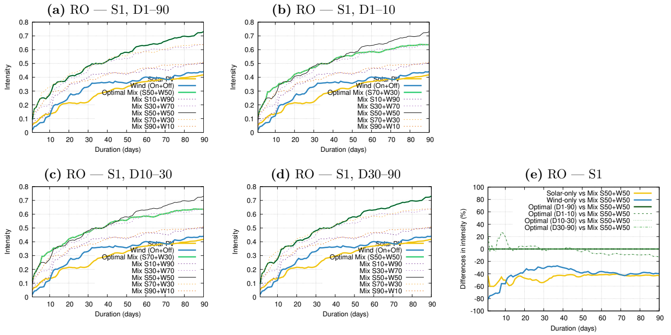
Figure 1. Panels (a–d): Intensity–Duration (ID) curves for renewable energy drought events of severity rank 1 ( S=1 ) in Romania (RO). Solar-only (yellow), wind-only (blue), and mixed capacity factor (CF) combinations are shown, with the optimal mix in green and the 50–50 mix in black (other combinations are displayed by dashed lines). Each panel shows the optima for different duration ranges: (a) D1–90, (b) D1–10, (c) D10–30 and (d) D30–90. Panel (e) displays the corresponding relative differences in drought intensity (%) between different renewable deployment configurations and the reference 50–50 solar–wind mix. Yellow and blue curves show differences between the solar-only and wind-only cases, respectively, and the 50–50 mix. Green curves show differences between the optimal mixes obtained for the four different optimized duration intervals (D1–90, D1–10, D10–30, and D30–90) and the 50–50 mix. Positive values indicate cases in which the 50–50 mix yields higher drought intensity (performs worse) than the corresponding reference configuration, while negative values indicate the opposite.
