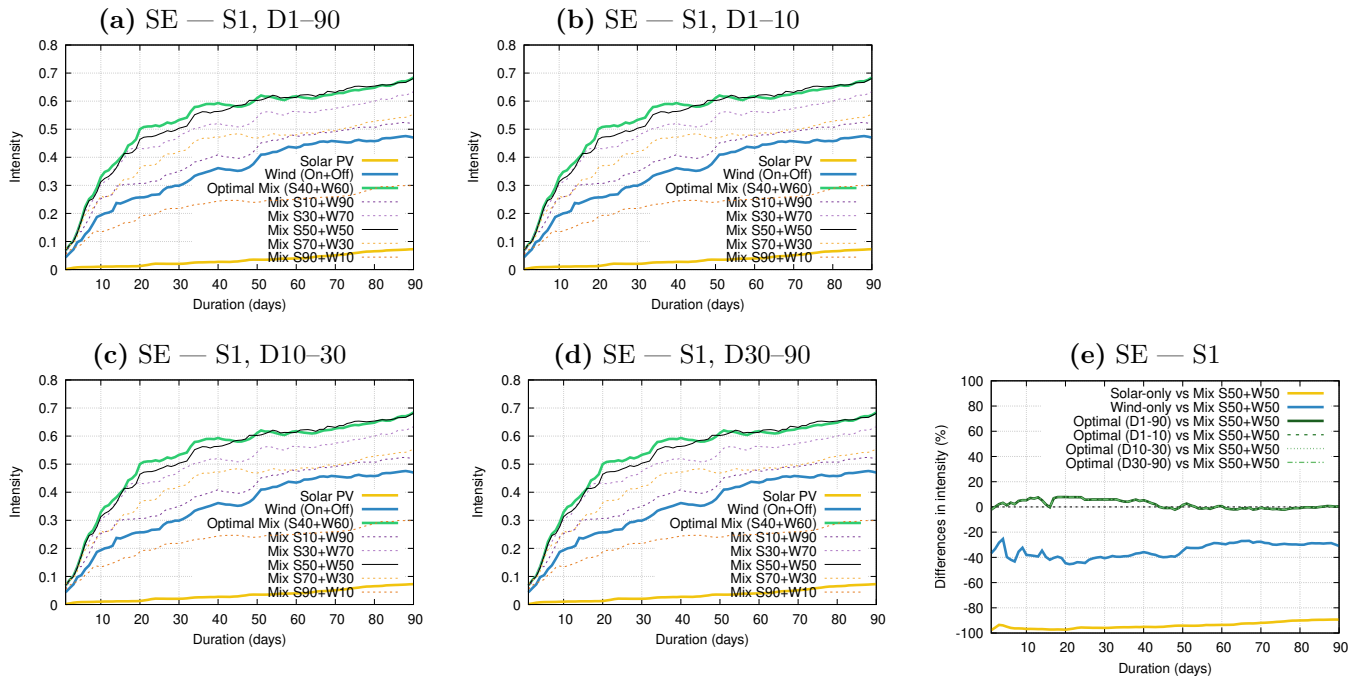
Figure 1. Panels (a–d): Intensity–Duration (ID) curves for renewable energy drought events of severity rank 1 ( S=1 ) in Sweden (SE). Solar-only (yellow), wind-only (blue), and mixed capacity factor (CF) combinations are shown, with the optimal mix in green and the 50–50 mix in black (other combinations are displayed by dashed lines). Each panel shows the optima for different duration ranges: (a) D1–90, (b) D1–10, (c) D10–30 and (d) D30–90. Panel (e) displays the corresponding relative differences in drought intensity (%) between different renewable deployment configurations and the reference 50–50 solar–wind mix. Yellow and blue curves show differences between the solar-only and wind-only cases, respectively, and the 50–50 mix. Green curves show differences between the optimal mixes obtained for the four different optimized duration intervals (D1–90, D1–10, D10–30, and D30–90) and the 50–50 mix. Positive values indicate cases in which the 50–50 mix yields higher drought intensity (performs worse) than the corresponding reference configuration, while negative values indicate the opposite.
