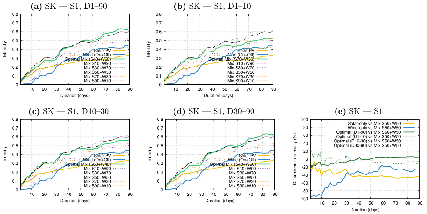
Figure 1. Panels (a–d): Intensity–Duration (ID) curves for renewable energy drought events of severity rank 1 ( S=1 ) in Slovakia (SK). Solar-only (yellow), wind-only (blue), and mixed capacity factor (CF) combinations are shown, with the optimal mix in green and the 50–50 mix in black (other combinations are displayed by dashed lines). Each panel shows the optima for different duration ranges: (a) D1–90, (b) D1–10, (c) D10–30 and (d) D30–90. Panel (e) displays the corresponding relative differences in drought intensity (%) between different renewable deployment configurations and the reference 50–50 solar–wind mix. Yellow and blue curves show differences between the solar-only and wind-only cases, respectively, and the 50–50 mix. Green curves show differences between the optimal mixes obtained for the four different optimized duration intervals (D1–90, D1–10, D10–30, and D30–90) and the 50–50 mix. Positive values indicate cases in which the 50–50 mix yields higher drought intensity (performs worse) than the corresponding reference configuration, while negative values indicate the opposite.
