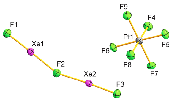
Figure 4. Asymmetric unit of [\text{Xe}_2\text{F}_3][\text{PtF}_6] , showing atom labeling. Ellipsoids are drawn at the 50% probability level.
