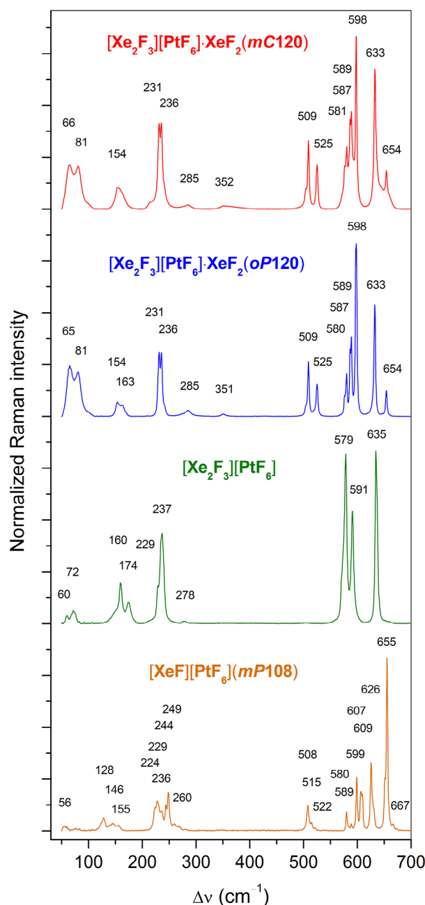
Figure 6. Low-temperature (100 K) Raman spectra of [\text{Xe}_2\text{F}_3][\text{PtF}_6]\cdot\text{XeF}_2(m\text{C120}) , [\text{Xe}_2\text{F}_3][\text{PtF}_6]\cdot\text{XeF}_2(o\text{P120}) , [\text{Xe}_2\text{F}_3][\text{PtF}_6] , and [\text{XeF}][\text{PtF}_6](m\text{P108}) .
