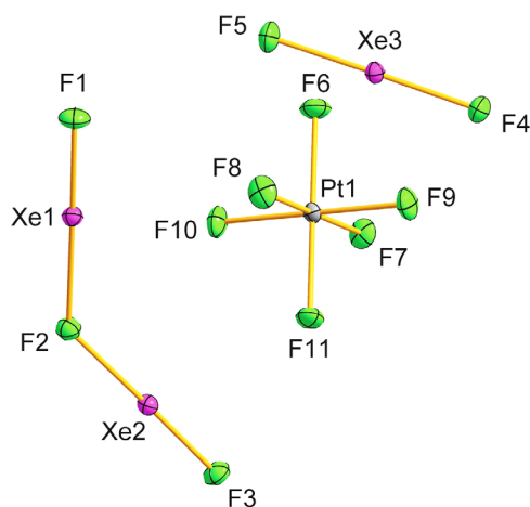
Figure 2. Asymmetric unit of [Xe 2 F 3 ][PtF 6 ].XeF 2 ( mC120 ), showing atom labeling. Ellipsoids are drawn at the 50% probability level.
