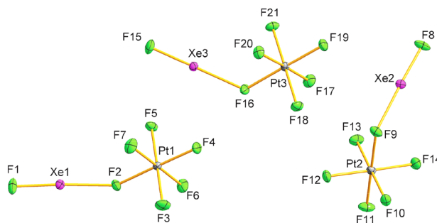
Figure 5. Asymmetric unit of [\text{XeF}][\text{PtF}_6] , featuring the three symmetry-inequivalent units and showing atom labeling. Ellipsoids are drawn at the 50% probability level.
